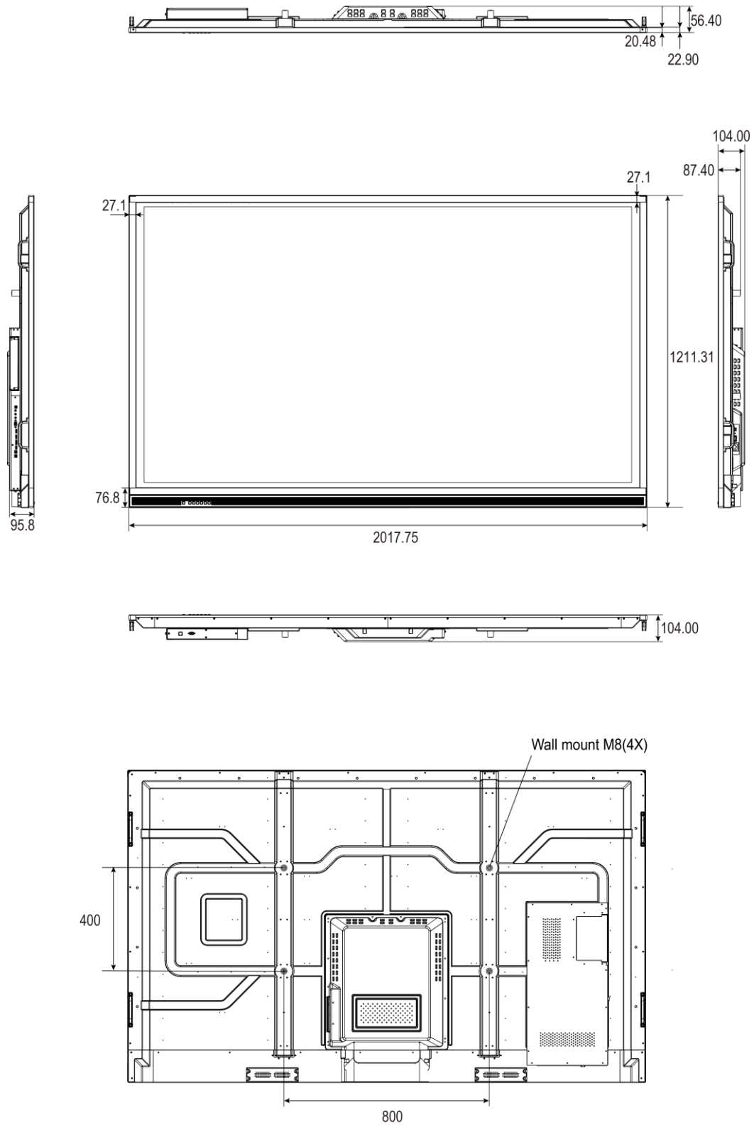
Figure 7-2. AVE-8620 Display Dimensions (mm)
