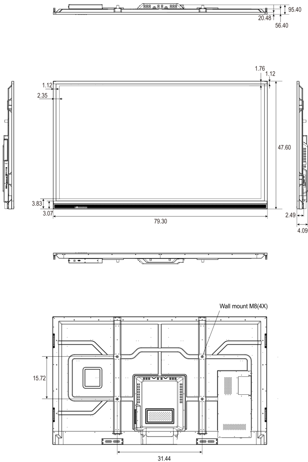
Figure 7-1. AVE-8620 Display Dimensions (inch)
