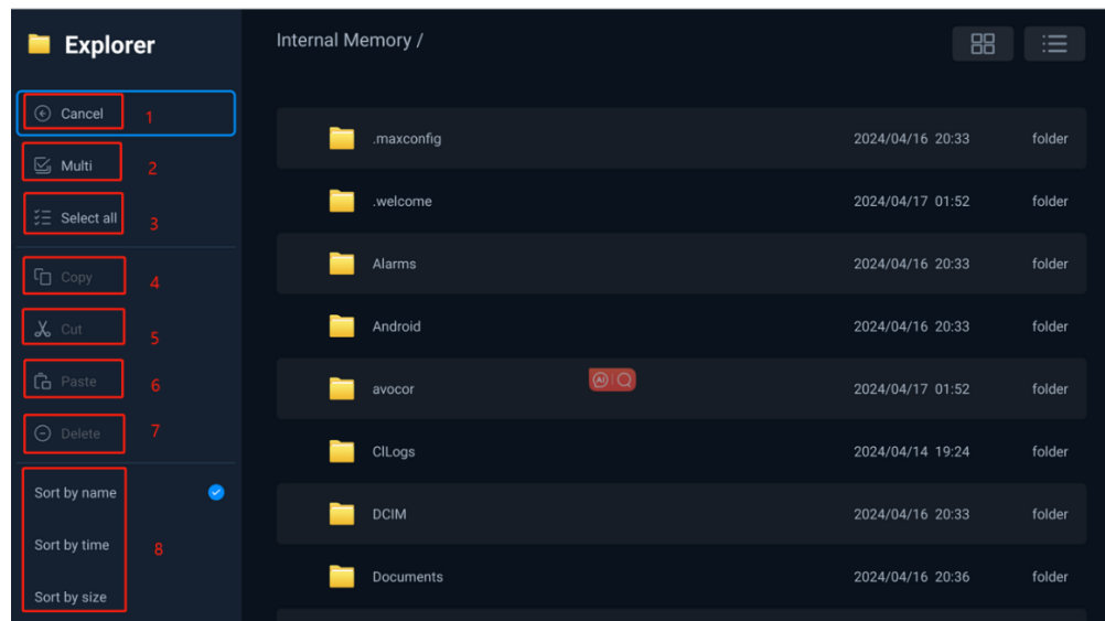
Explorer Menu
