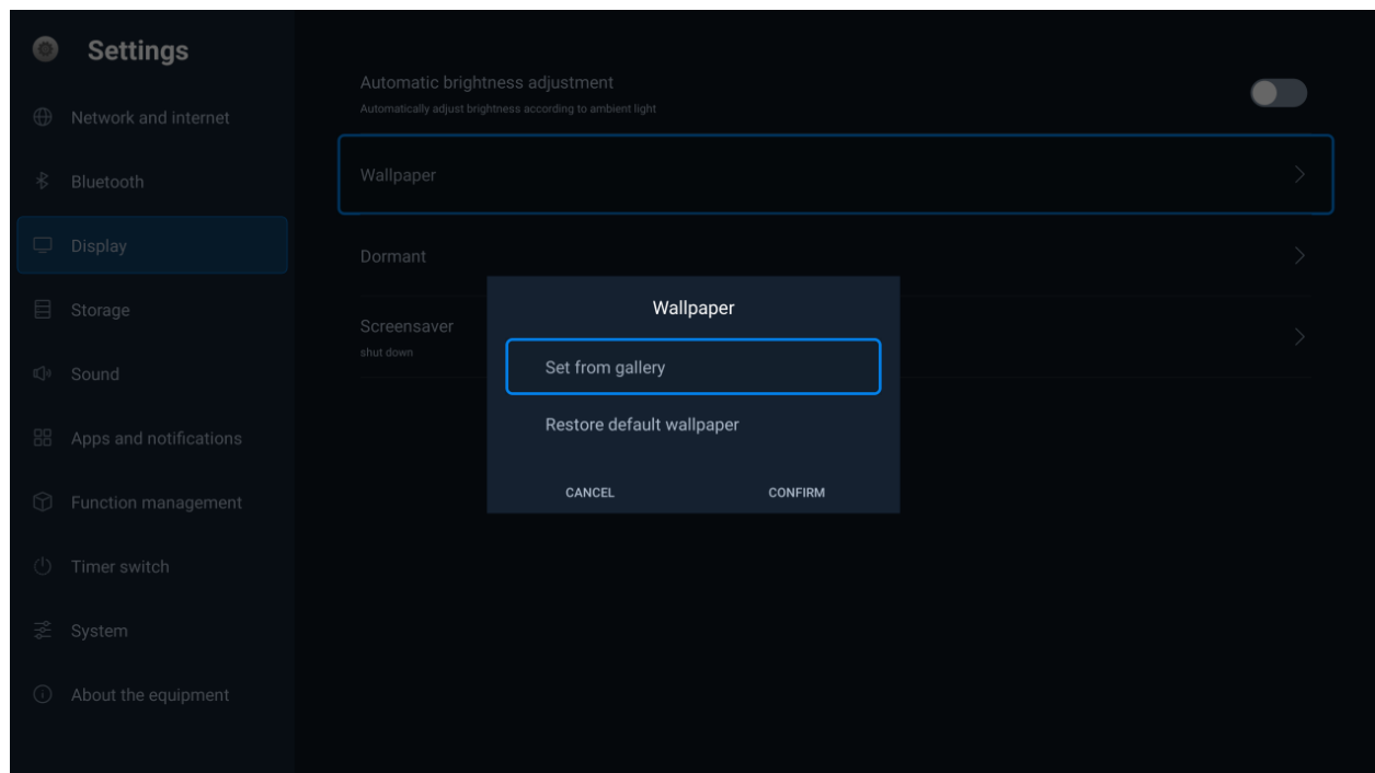
Wallpaper
