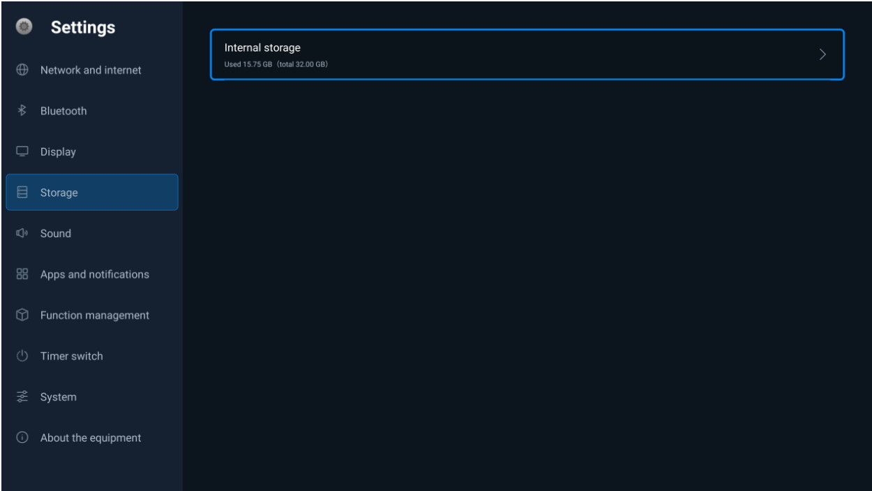
Storage
