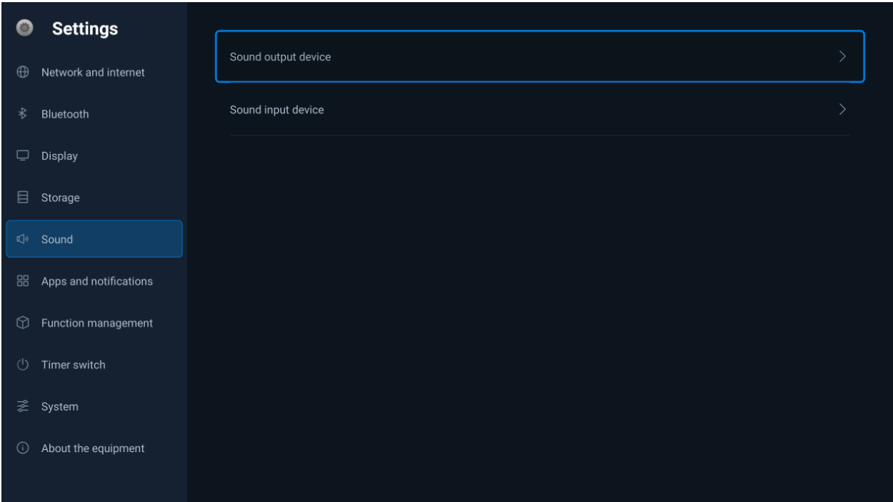
Sounds
