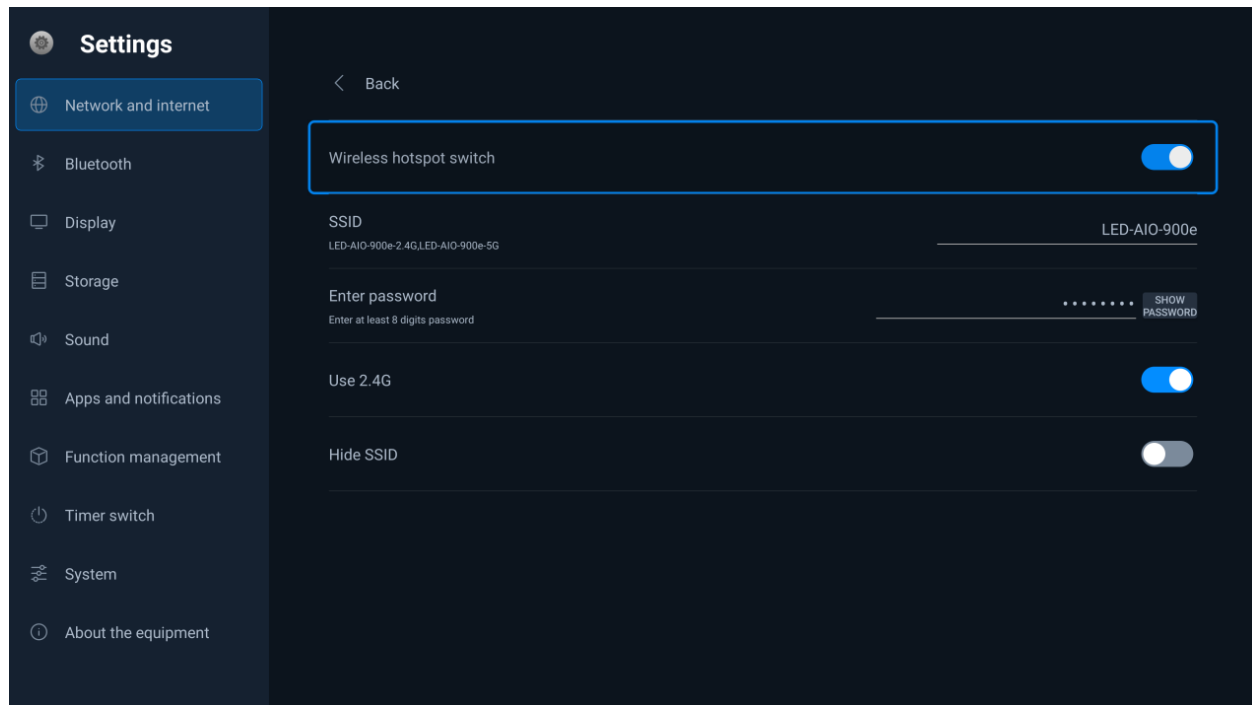
Portable Hotspots
